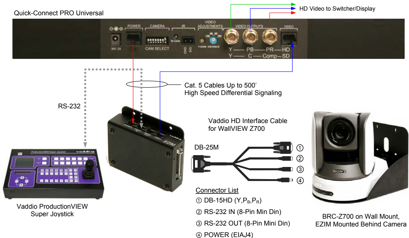
Figure 4: Basic system connectivity of a WallVIEW PRO Z700 System and ProductionVIEW™ Super Joystick Controller
