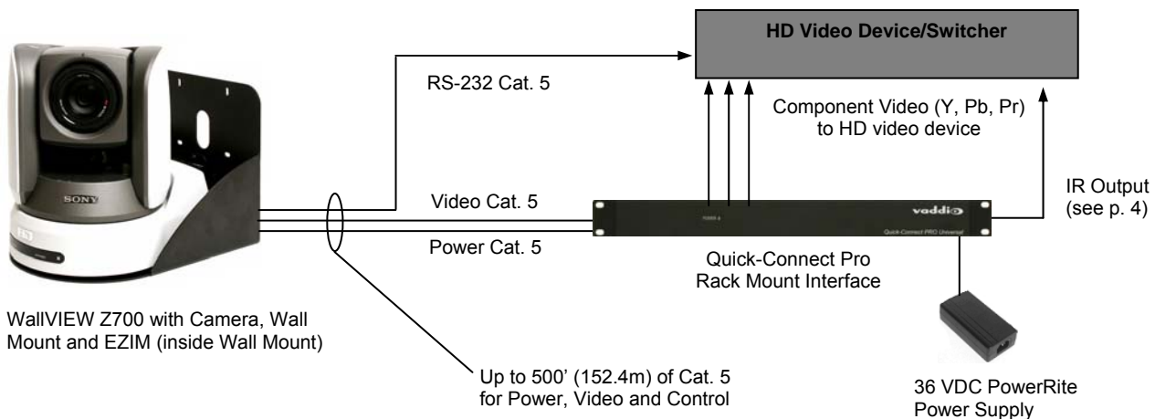
Figure 2: Basic connectivity of the WallVIEW PRO HD-700 System.
