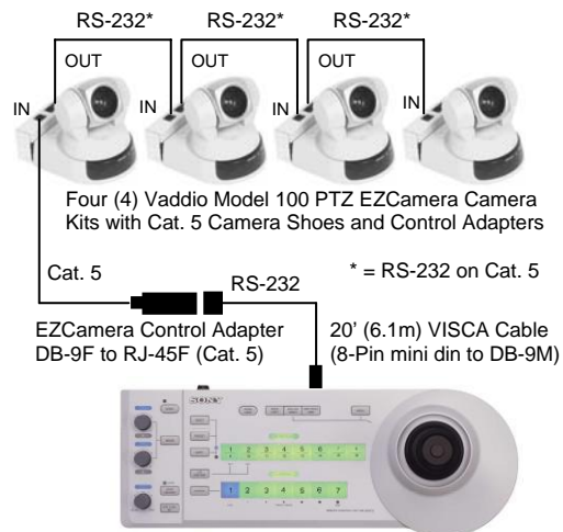
Figure 3: Sony Joystick with four (4) Camera Daisy Chain Control
