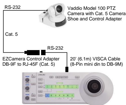
Figure 2: Sony RM-BR300 Joystick with Single Camera Control
