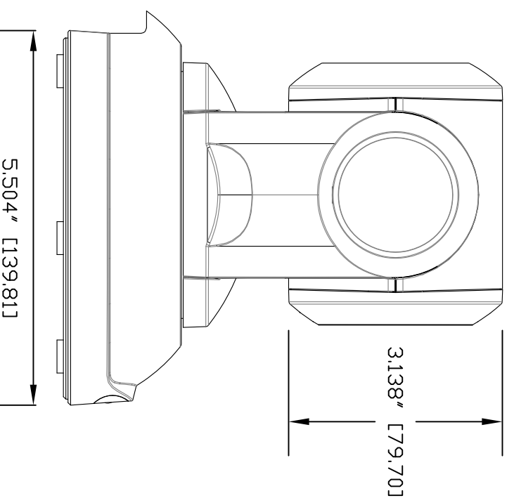
SIDE VIEW 1
