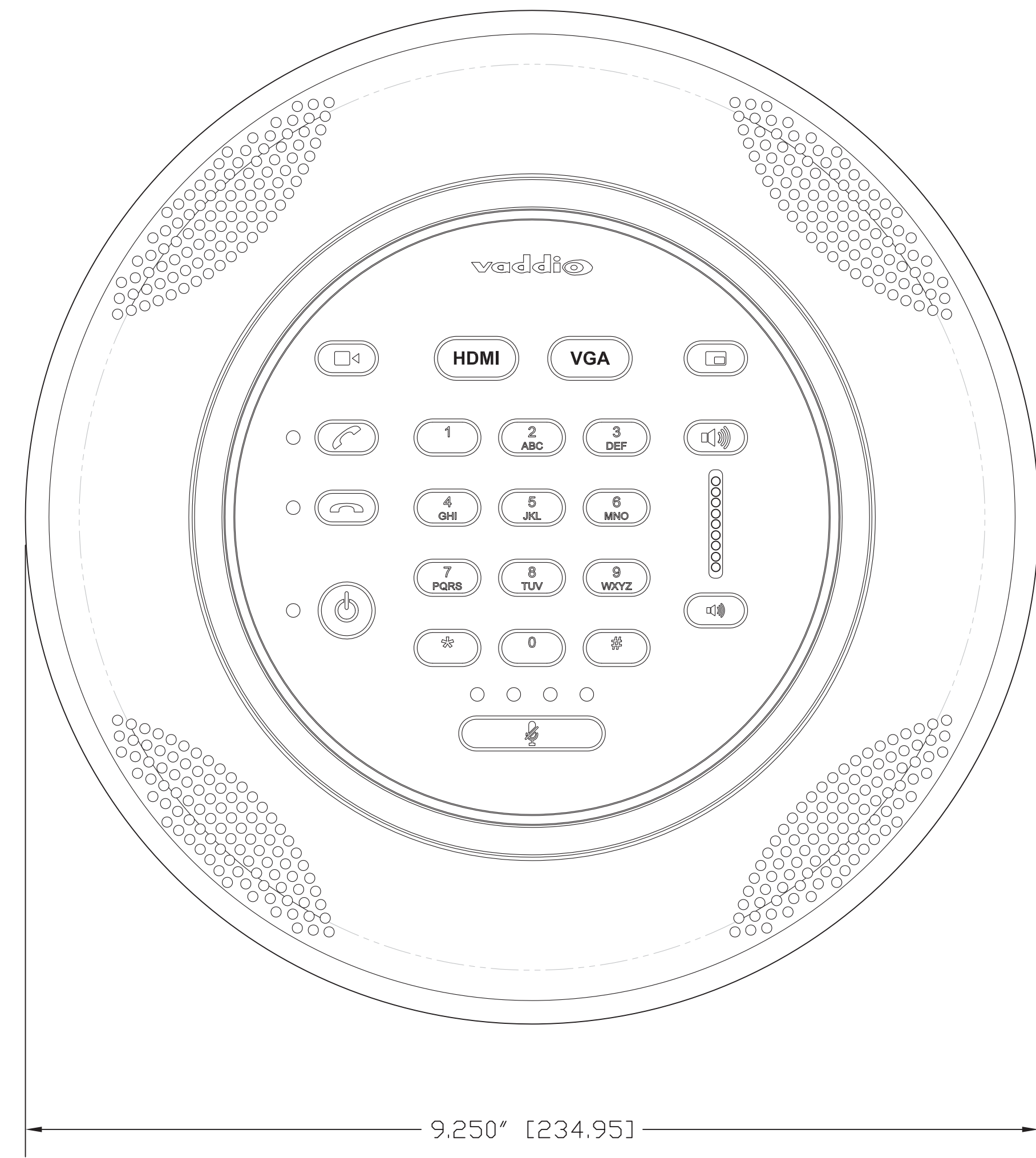
TOP VIEW
