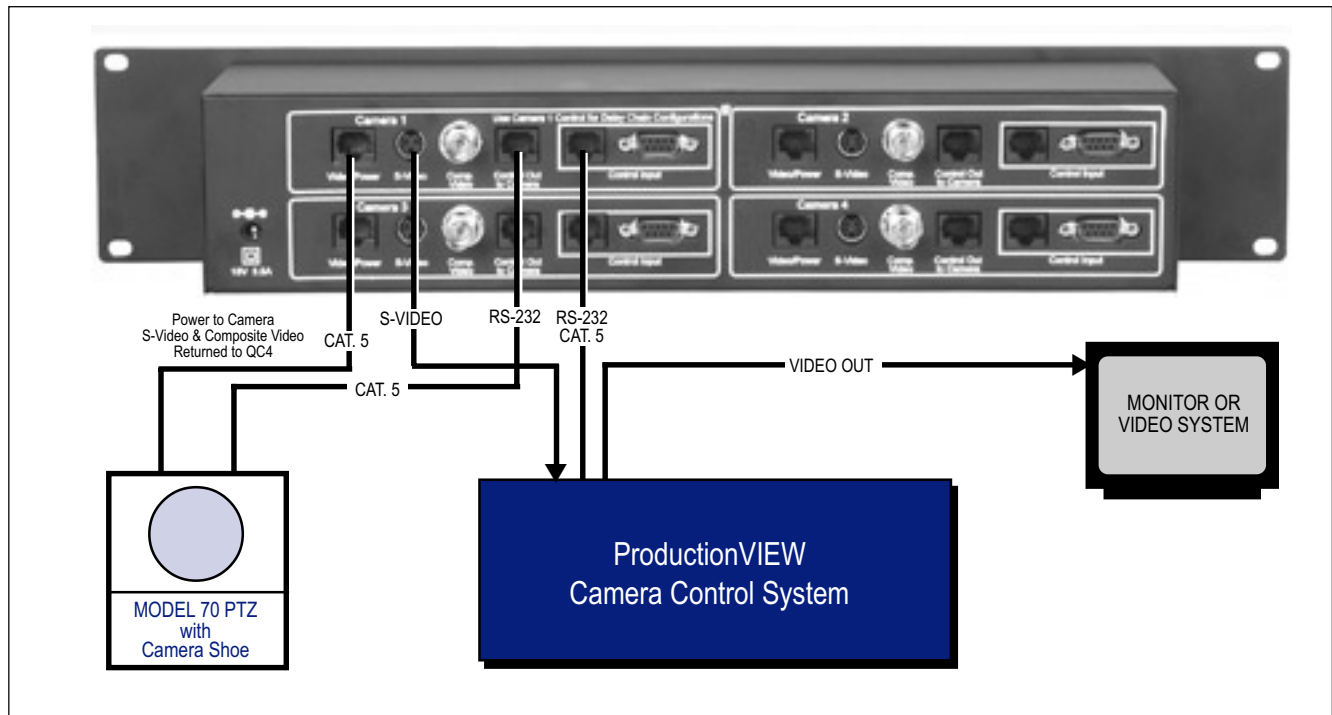
Figure 1 – Quick-Connect 4 back panel and Camera Port 1.
