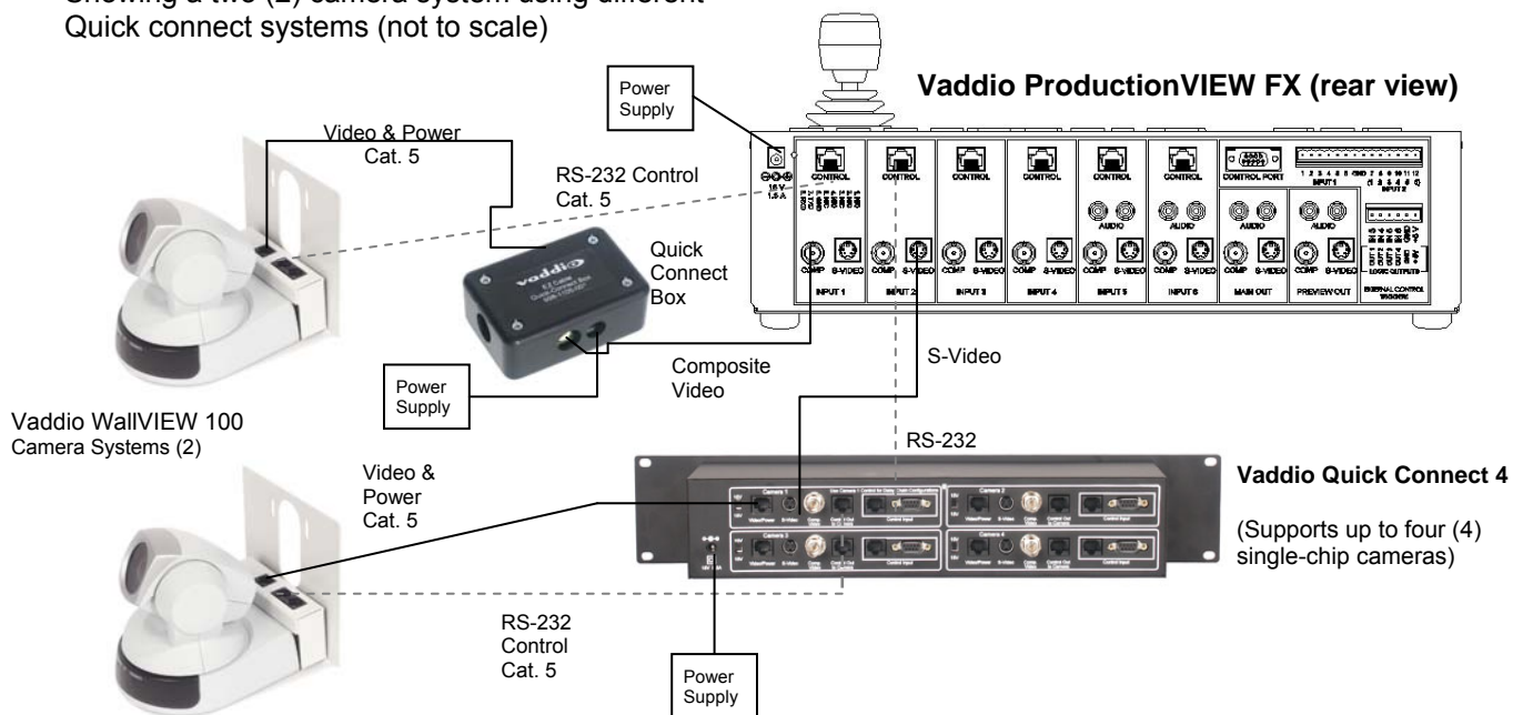
Figure 4: Basic Quick Configuration
