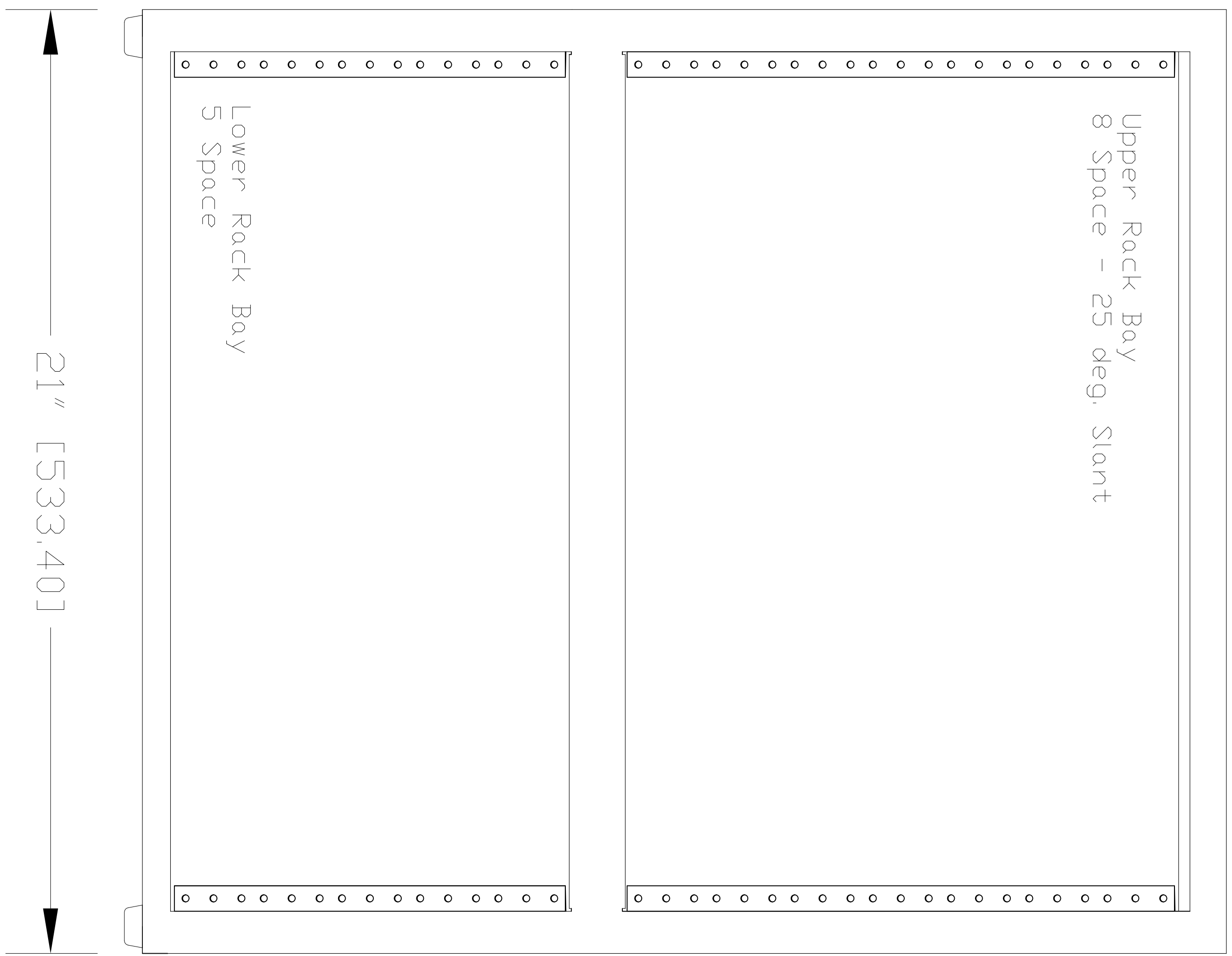
FRONT VIEW
