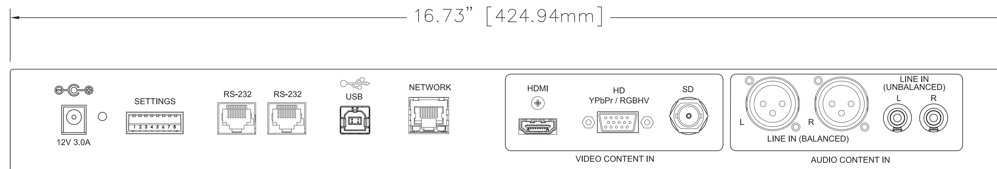
REAR PANEL CONNECTIONS
