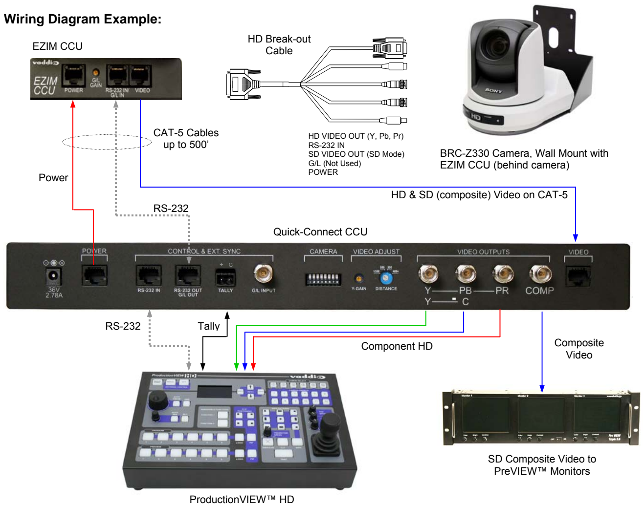
Figure 2: The WallVIEW CCU System uses a Cat. 5 (all 4-pairs) for power to ensure the motors receive the required current to operate properly. The Video Cat. 5 cable uses all four pairs for video. The RS-232 Cat. 5 provides communication to the camera for CCU and PTZ control and G/L (where applicable) to the camera. These Cat. 5 cables can be run up to 500' (152.4m). See Appendix 1 for wiring and pin-out information. NOTE: A direct RS-232 Cat. 5 cable is required for each Quick-Connect CCU and camera. Daisy-Chain configurations are not supported with Quick-Connect CCU.
