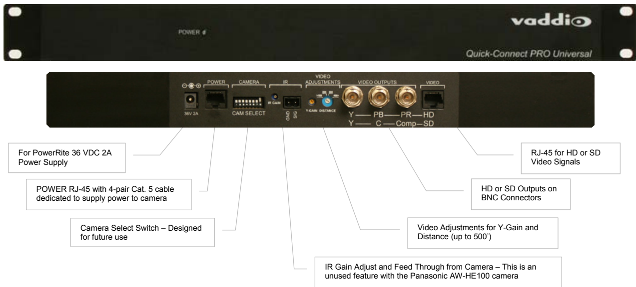
Figure 2: Quick-Connect PRO Interface front panel and rear panel images with functional callouts.
