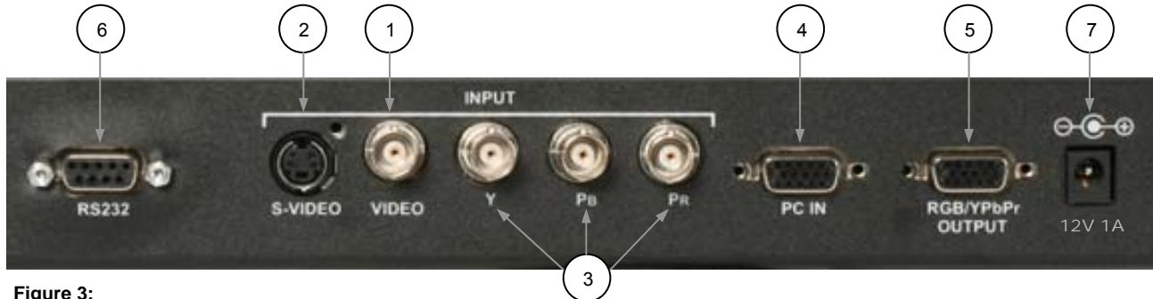
Figure 3: Rear Panel of the ProductionVIEW PC Expander
